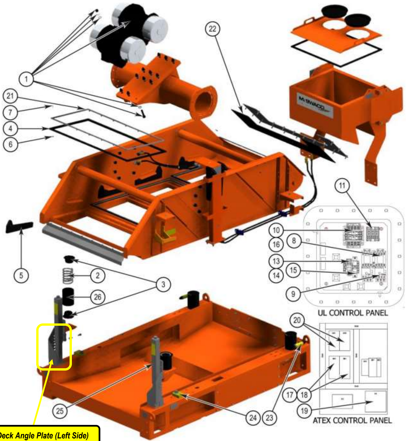
Figure 36. MONGOOSE PRO Shale Shaker Components Exploded View
